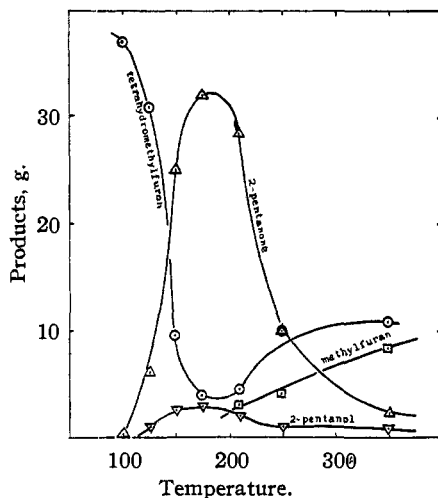
Fig. 1.—Products from methylfuran and hydrogen over a nickel catalyst at various temperatures. Each point corresponds with the passage of 41 g. of methylfuran and 80 liters of hydrogen over the catalyst in two hours.
